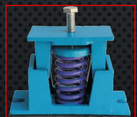
SPRING HANGAR/ VIBRATION ISOLATOR, SEISMIC RESTRAINTS& ISOLATION PADS (CANADA)
